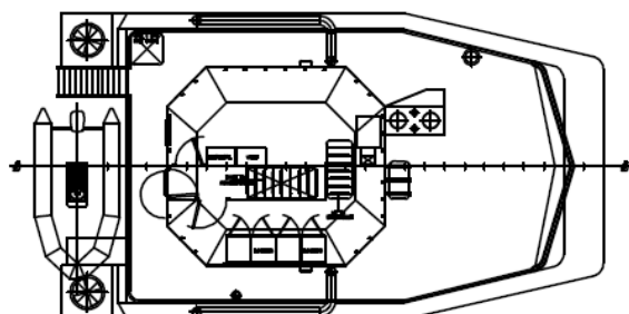
BOAT DECK
