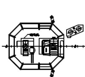
WHEELHOUSE DECK
